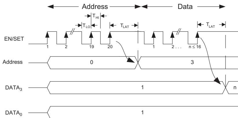
Figure 2: AS 2 Cwire Serial Interface Timing.
