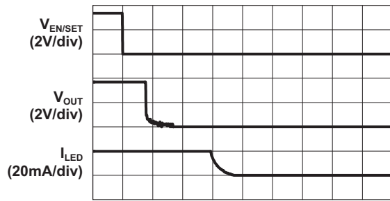
Time (100µs/div)
