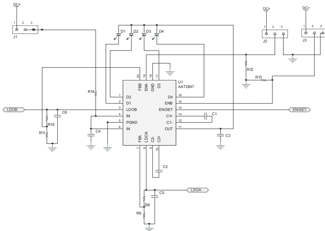
Figure 7: AAT2847 Section Schematic.
